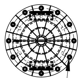
12 x M36 on \varnothing 900mm PCD
