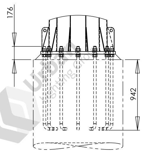
12 x M36 on \varnothing 900mm PCD
